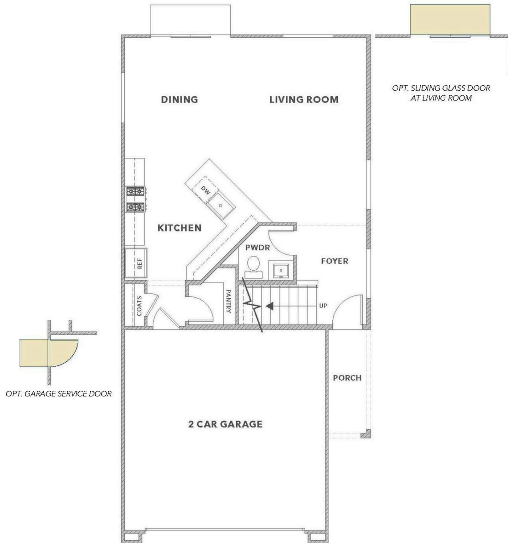
FIRST FLOOR
